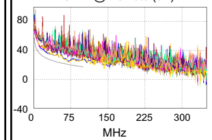
ACR-N @ Remote (dB)
