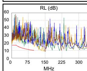
RL @ Remote (dB)
