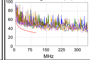
ACR-F @ Remote (dB)
