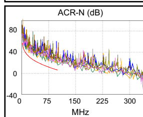
ACR-N @ Remote (dB)
