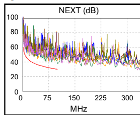
NEXT @ Remote (dB)
