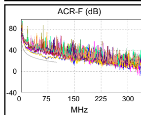
ACR-F @ Remote (dB)
